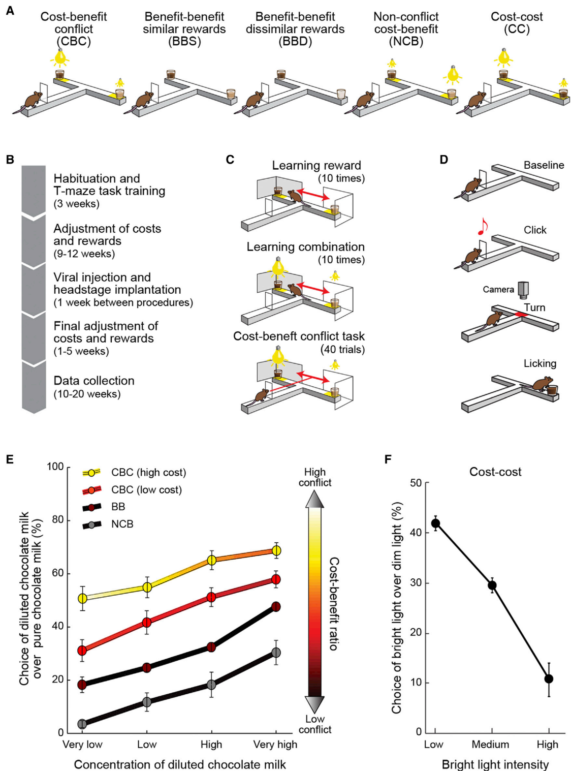
Figure 1. Decision-Making Tasks
